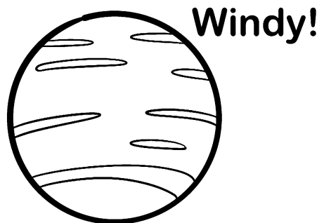
Neptune
